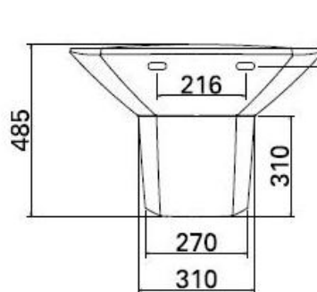
Pedestal Model : 105200
