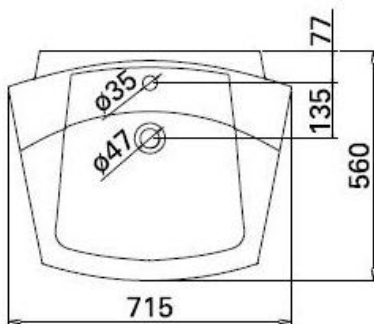
70 Wash Basin With Fixing Kit Model : 105320
