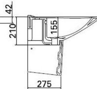
Trap Cover Model : 105220
